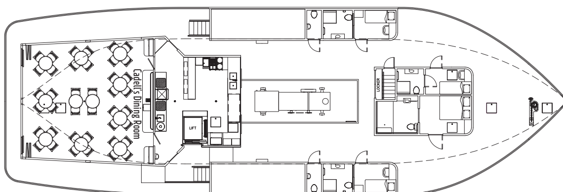
Main Deck
